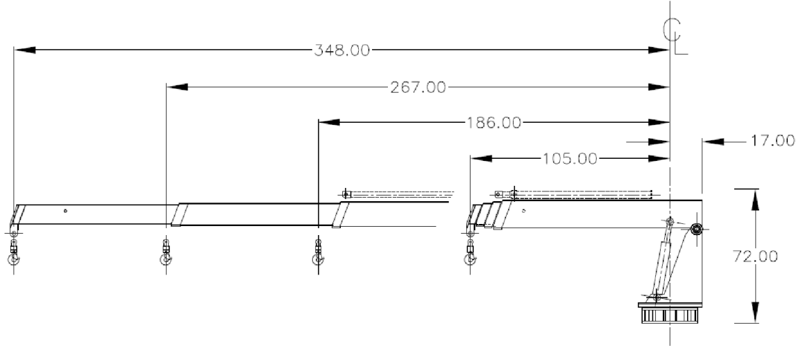
STANDARD ARA 208 CRANE 1500 LB @ 29'
