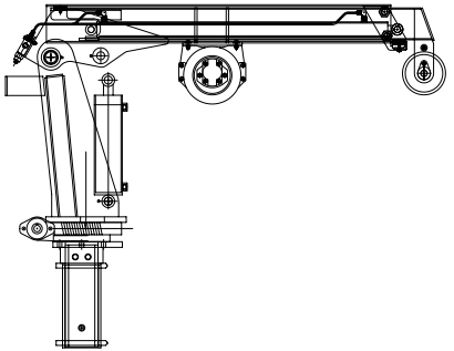
OPTIONAL MOVABLE, POCKET MOUNTED 2000 LB CRANE 120 VAC
