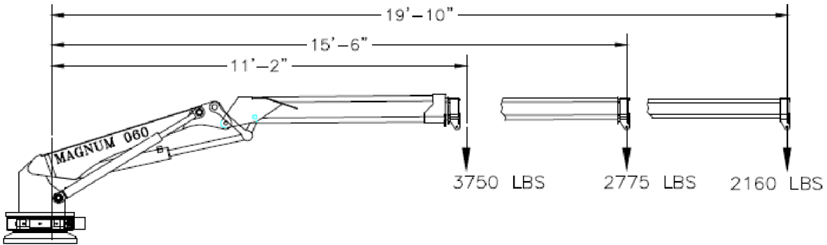
OPTIONAL MAGNUM KNUCKLE BOOM CRANE 2100 LB @ 20'
